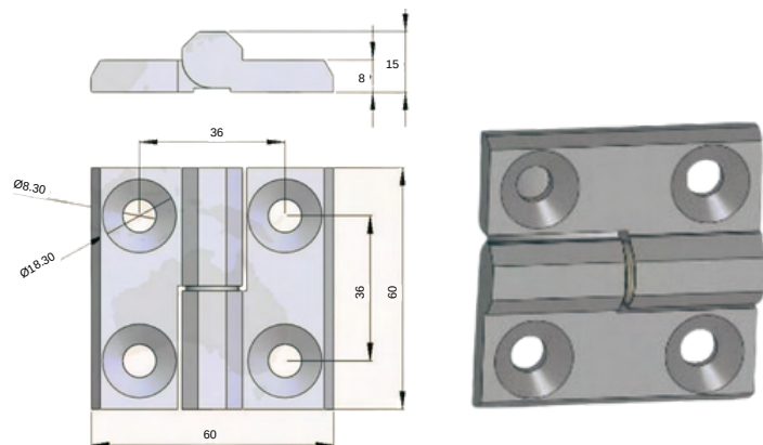
STAINLESS STEEL HINGE 2715-HT-6.5
