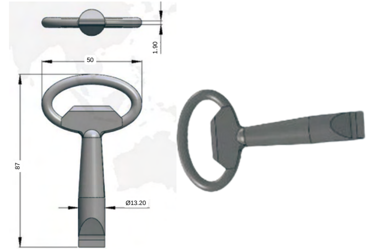
STAINLESS STEEL KEY
