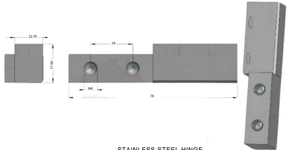
STAINLESS STEEL HINGE 3140-HT-1.1
