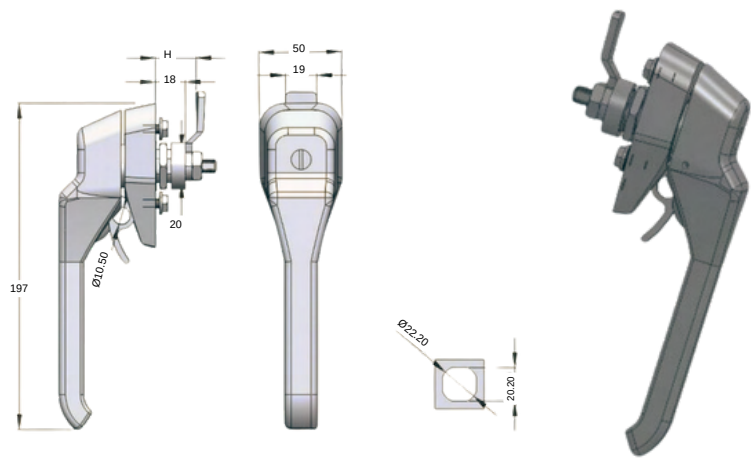
STAINLESS STEEL CYLINDER 2310-HT-4.2
