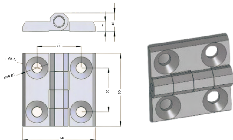
STAINLESS STEEL HINGE 2715-HT-6.1
