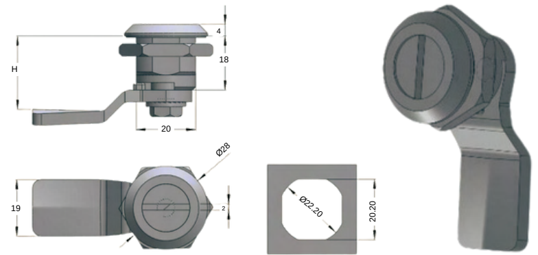
STAINLESS STEEL QUARTER TURN 2513-HT-1.1
