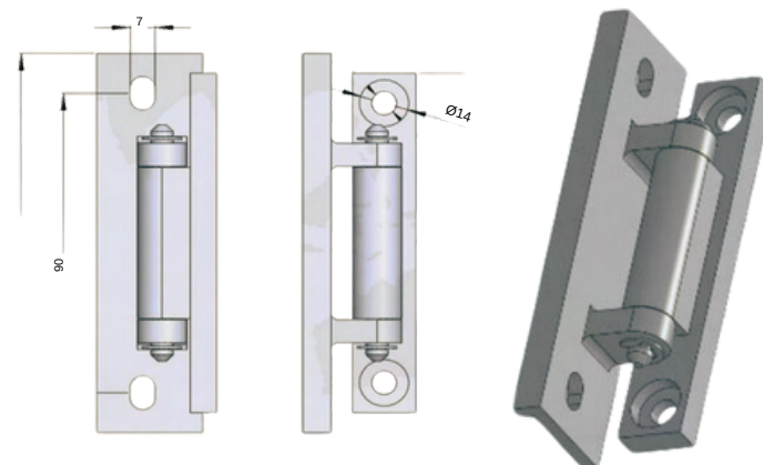
STAINLESS STEEL HINGE 3140-HT-1.28
