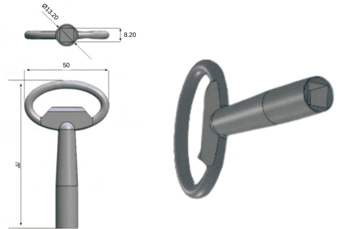
STAINLESS STEEL KEY
