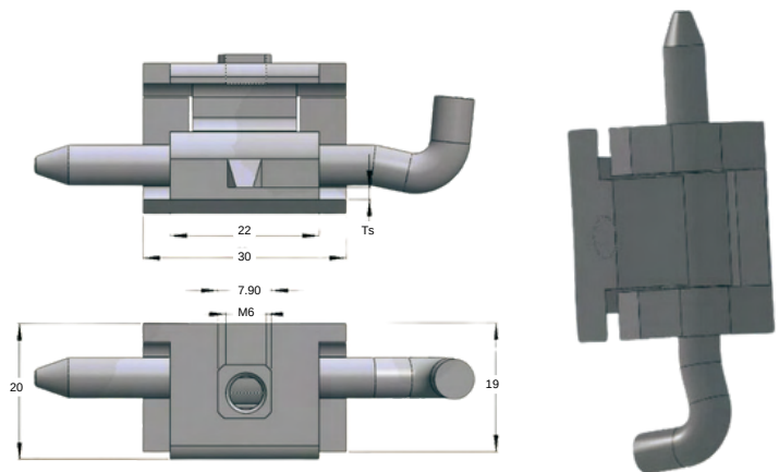
STAINLESS STEEL HINGE
