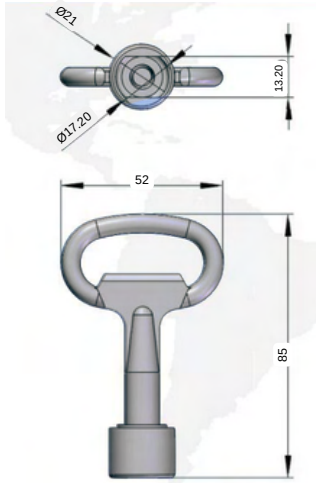
STAINLESS STEEL KEY
