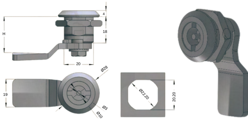
STAINLESS STEEL QUARTER TURN 2513-HT-2.1
