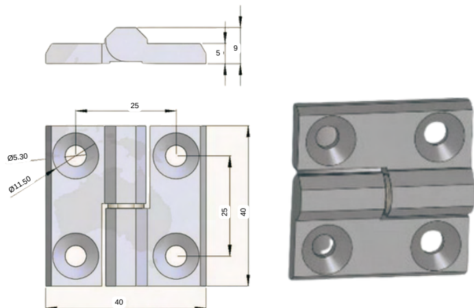
STAINLESS STEEL HINGE 2715-HT-4.3
