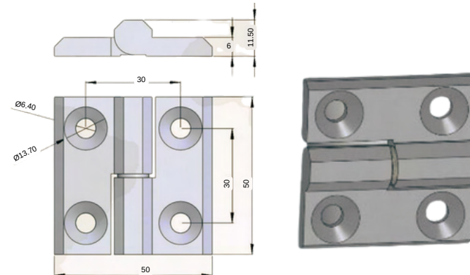
STAINLESS STEEL HINGE 2715-HT-5.5
