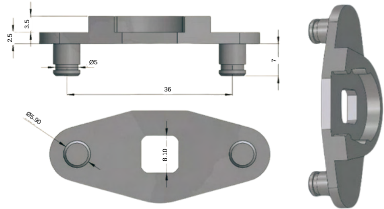
STAINLESS STEEL FITTINGS
