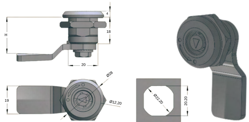
STAINLESS STEEL QUARTER TURN 2513-HT-1.4
