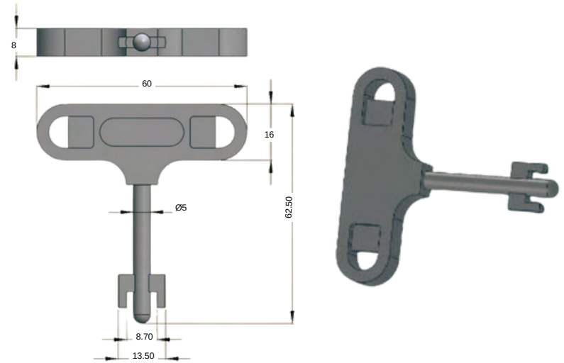
STAINLESS STEEL KEY
