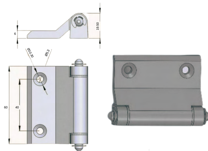
STAINLESS STEEL HINGE
