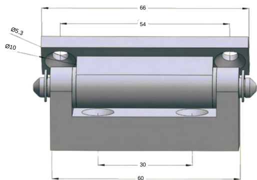
STAINLESS STEEL HINGE
