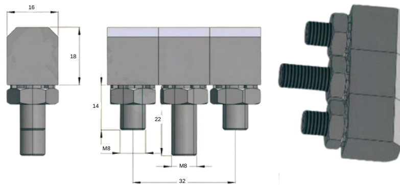
STAINLESS STEEL HINGE 3140-HT-1.5
