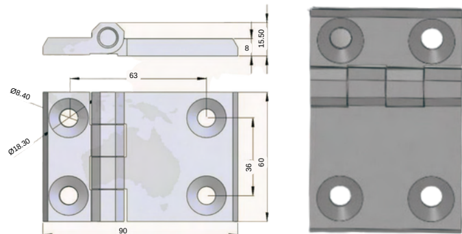
STAINLESS STEEL HINGE 2715-HT-6.2
