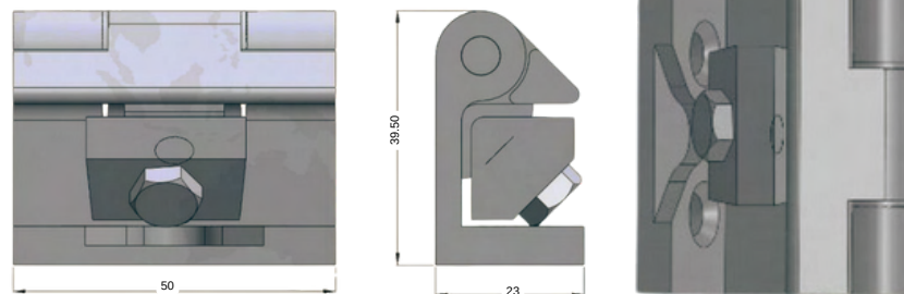
STAINLESS STEEL HINGE 3140-HT-1.24
