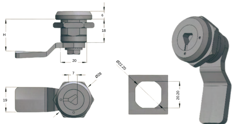
STAINLESS STEEL QUARTER TURN 2514-HT-3.1
