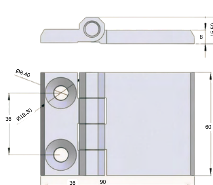
STAINLESS STEEL HINGE 2715-HT-6.8
