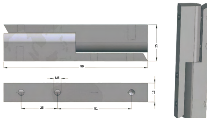
STAINLESS STEEL HINGE 3140-HT-1.20
