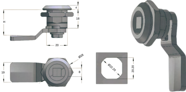
STAINLESS STEEL QUARTER TURN 2513-HT-4.3
