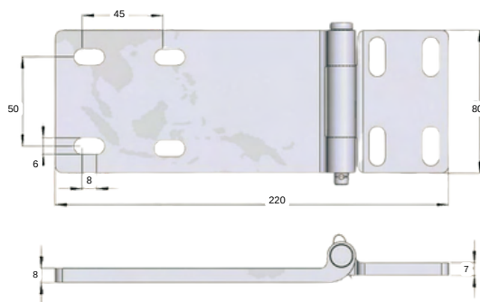
STAINLESS STEEL HINGE 2715-HT-8.1
