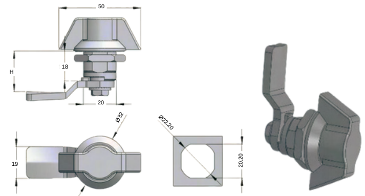
NON LOCKING HANDLE 2310-HT-3.3
