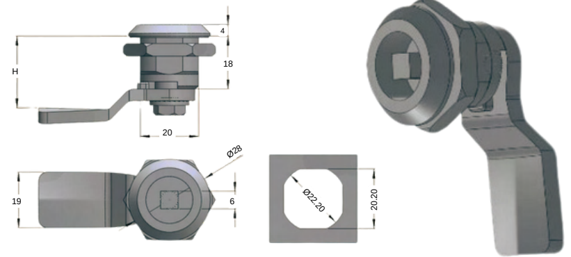
STAINLESS STEEL QUARTER TURN 2513-HT-4.1
