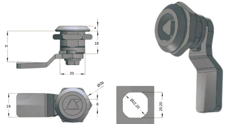
STAINLESS STEEL QUARTER TURN 2513-HT-3.2
