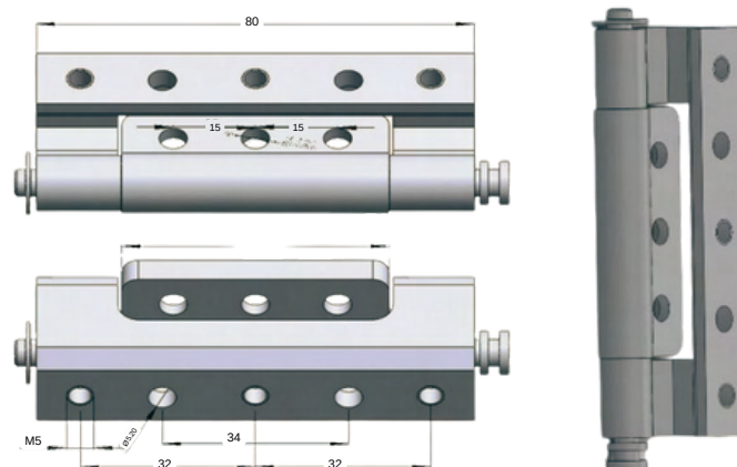
STAINLESS STEEL HINGE 3140-HT-1.21
