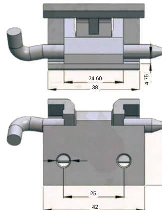
STAINLESS STEEL HINGE 3140-HT-1.13
