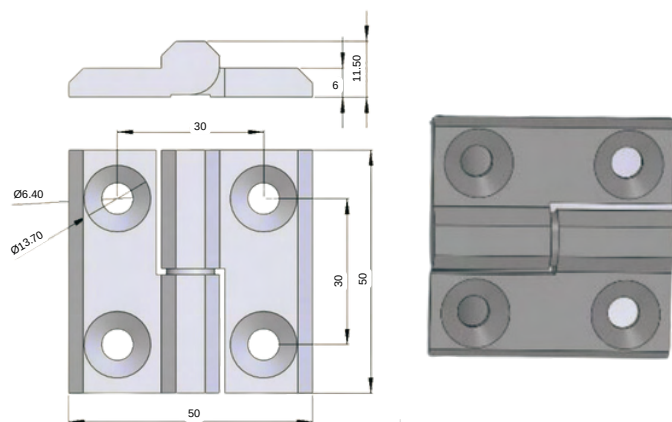
STAINLESS STEEL HINGE 2715-HT-5.4
