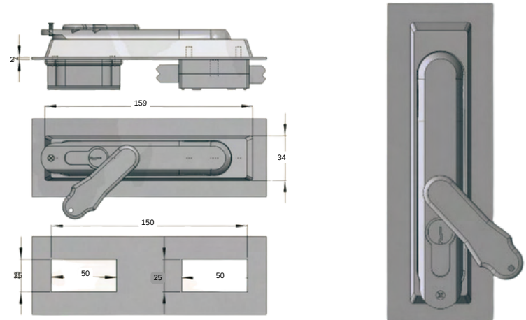
ZINC DIE-CAST CYLINDER 1810-HT-1.1
