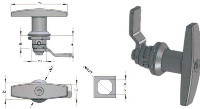
ZINC DIE-CAST CYLINDER | STAINLESS STEEL CYLINDER 2310-HT-2.1 | 2310-HT-2.2
