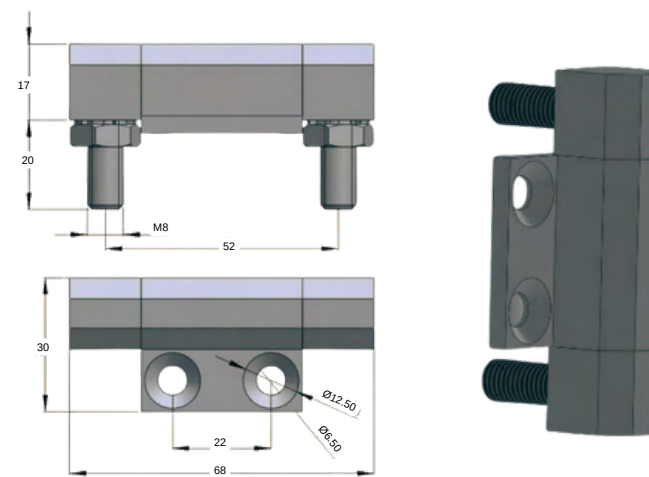
STAINLESS STEEL HINGE 3140-HT-1.10
