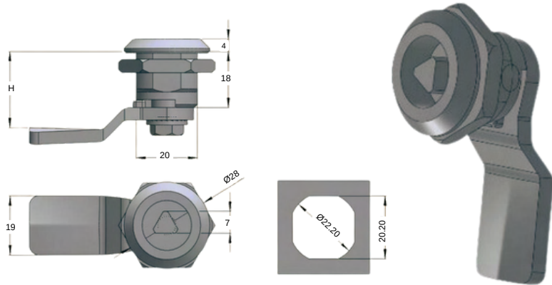
STAINLESS STEEL QUARTER TURN 2513-HT-3.1
