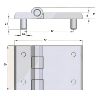
STAINLESS STEEL HINGE 2715-HT-6.7
