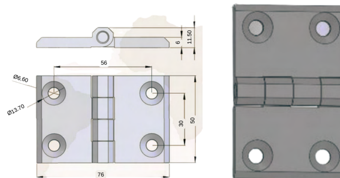
STAINLESS STEEL HINGE 2715-HT-5.2
