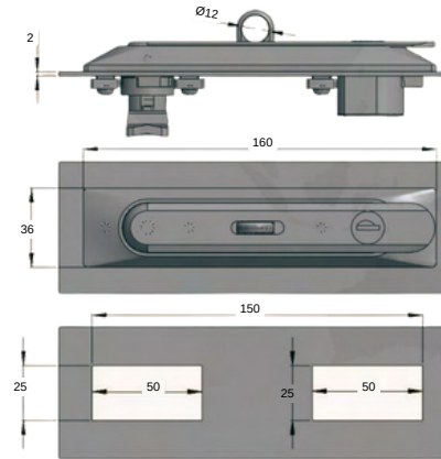
ZINC DIE-CAST CYLINDER 1810-HT-4.1
