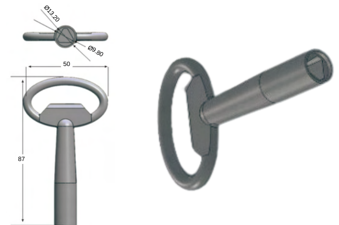
STAINLESS STEEL KEY
