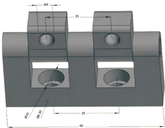
STAINLESS STEEL HINGE 3140-HT-1.27
