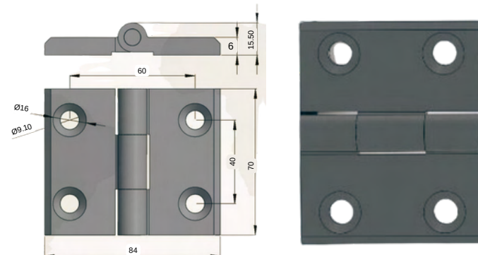
STAINLESS STEEL HINGE 2715-HT-7.1
