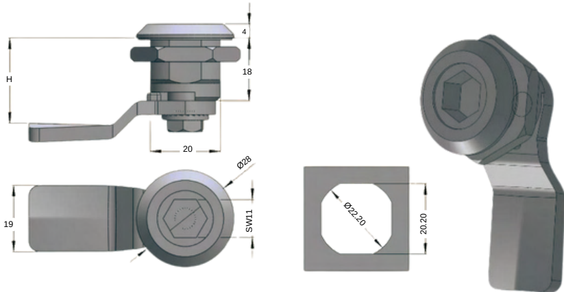
STAINLESS STEEL QUARTER TURN 2513-HT-6.2
