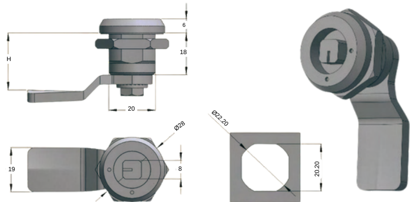
STAINLESS STEEL QUARTER TURN 2514-HT-4.2
