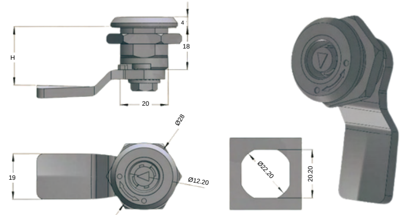
STAINLESS STEEL QUARTER TURN 2513-HT-1.3
