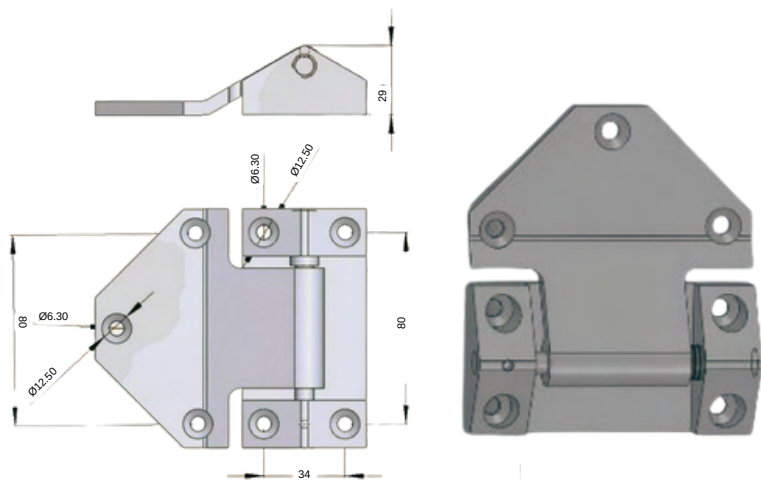
STAINLESS STEEL HINGE 3140-HT-1.18
