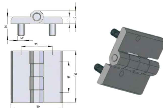
STAINLESS STEEL HINGE 2715-HT-6.6
