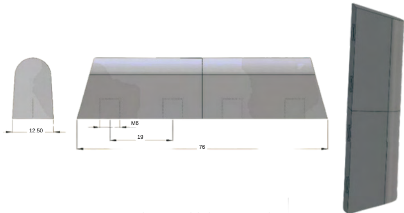
STAINLESS STEEL HINGE 3140-HT-1.3
