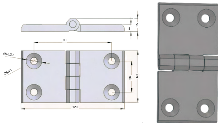
STAINLESS STEEL HINGE 2715-HT-6.3
