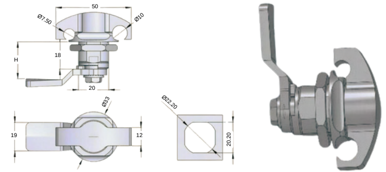
NON LOCKING HANDLE 2310-HT-5.1
