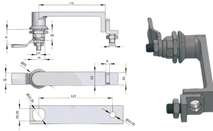
FOR PADLOCK 2310-HT-6.1
