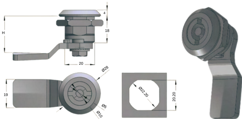
STAINLESS STEEL QUARTER TURN 2513-HT-2.2
