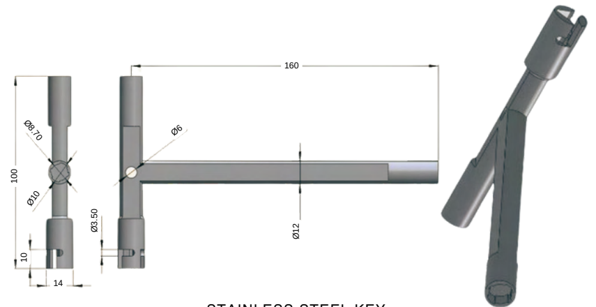
STAINLESS STEEL KEY
