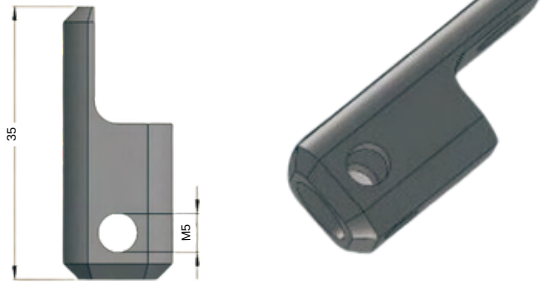
STAINLESS STEEL FITTINGS
