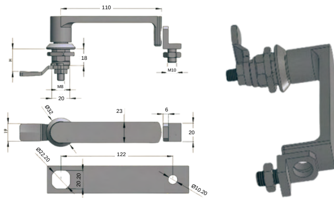
FOR PADLOCK 2310-HT-7.1
