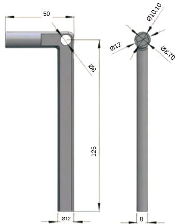
STAINLESS STEEL KEY
