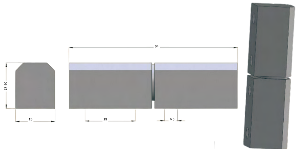
STAINLESS STEEL HINGE 3140-HT-1.2
