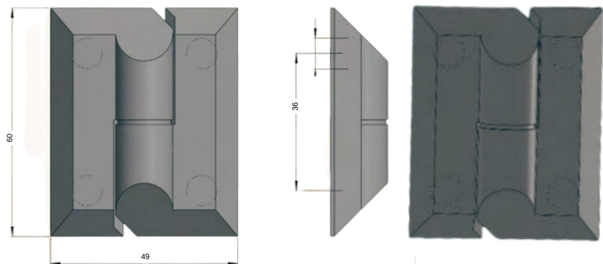
STAINLESS STEEL HINGE 3140-HT-1.19
