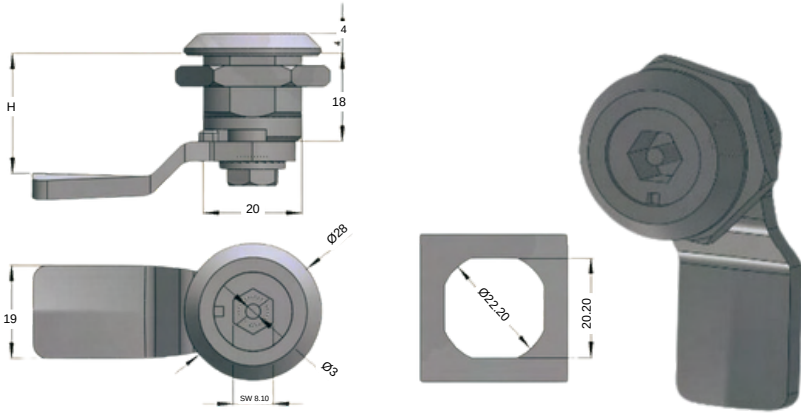
STAINLESS STEEL QUARTER TURN 2513-HT-6.1
