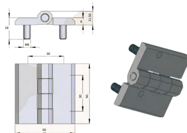
STAINLESS STEEL HINGE 2715-HT-5.6
