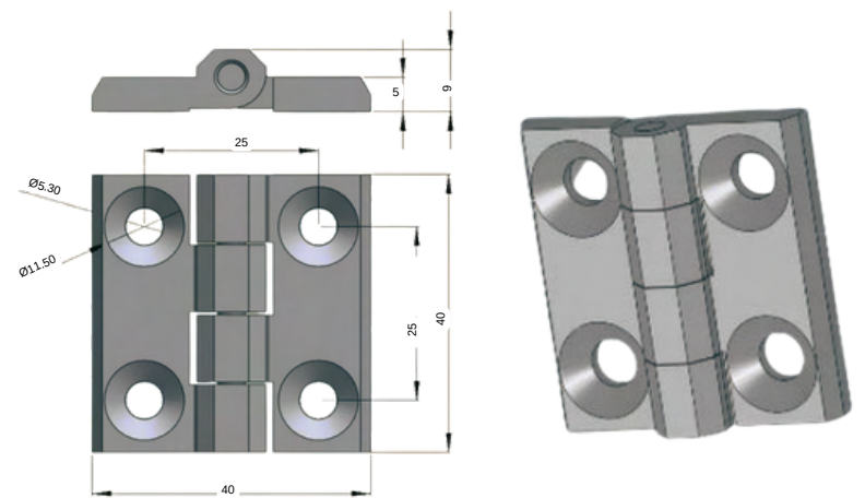
STAINLESS STEEL HINGE 2715-HT-4.1
