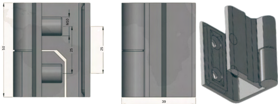
STAINLESS STEEL HINGE 3140-HT-1.22
