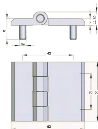
STAINLESS STEEL HINGE 2715-HT-5.8
