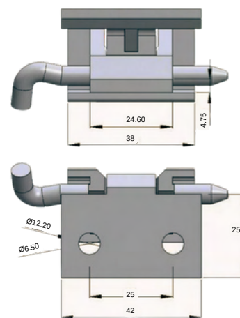
STAINLESS STEEL HINGE 3140-HT-1.14
