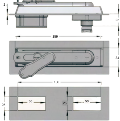
ZINC DIE-CAST CYLINDER 1810-HT-3.1
