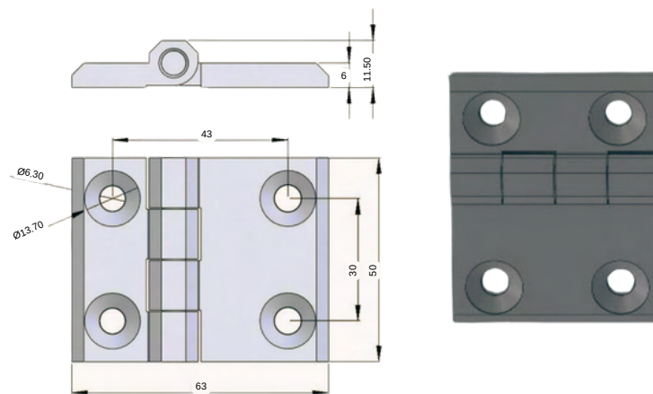
STAINLESS STEEL HINGE 2715-HT-5.3
