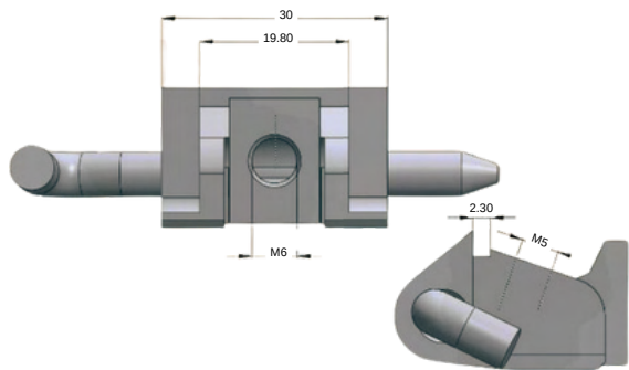
STAINLESS STEEL HINGE 3140-HT-1.11
