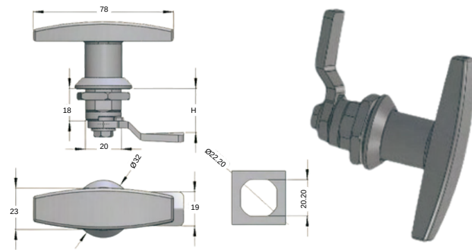
NON LOCKING HANDLE 2310-HT-2.3
