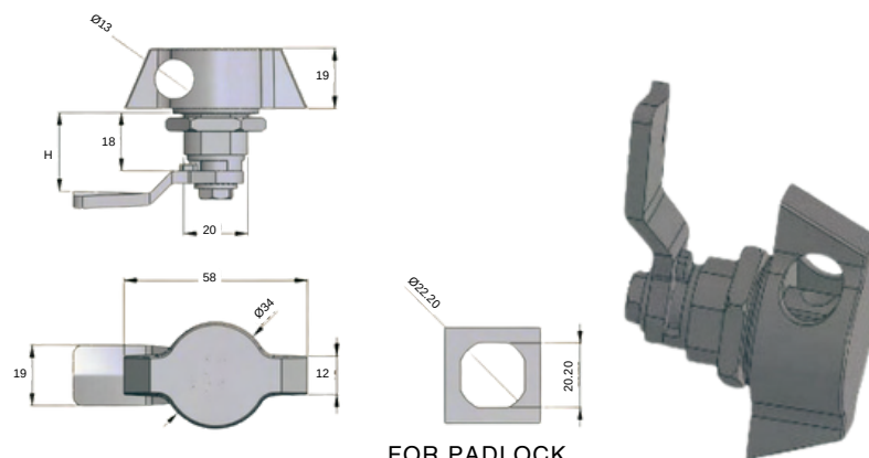
FOR PADLOCK 2310-HT-17.1
