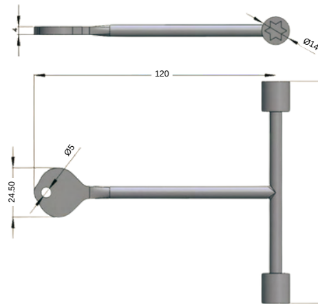
STAINLESS STEEL KEY
