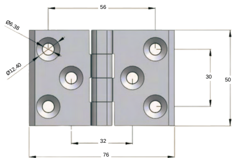
STAINLESS STEEL HINGE 2715-HT-3.2
