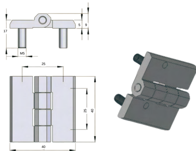
STAINLESS STEEL HINGE 2715-HT-4.4
