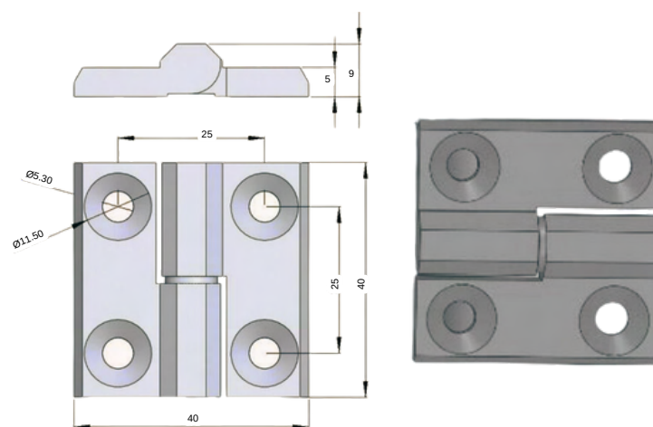
STAINLESS STEEL HINGE 2715-HT-4.2
