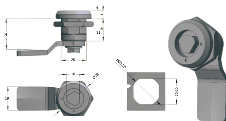
STAINLESS STEEL QUARTER TURN 2514-HT-3.3
