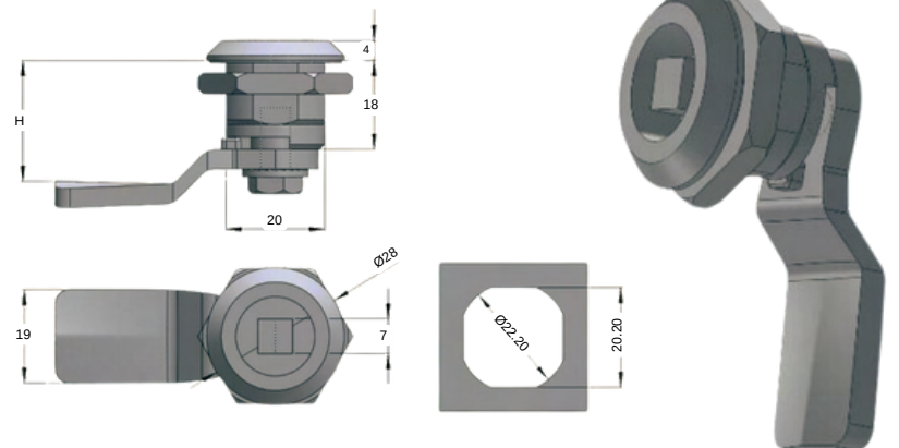
STAINLESS STEEL QUARTER TURN 2513-HT-4.2
