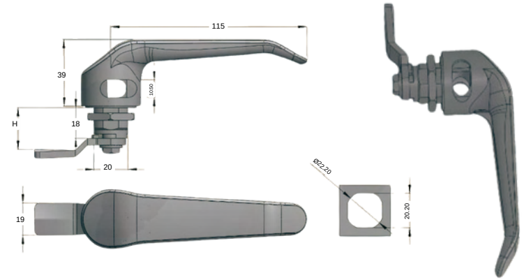
FOR PADLOCK 2310-HT-8.1
