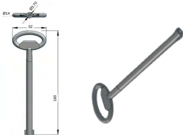
STAINLESS STEEL KEY
