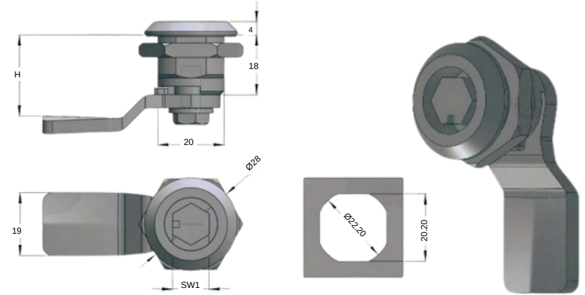
STAINLESS STEEL QUARTER TURN 2513-HT-6.3
