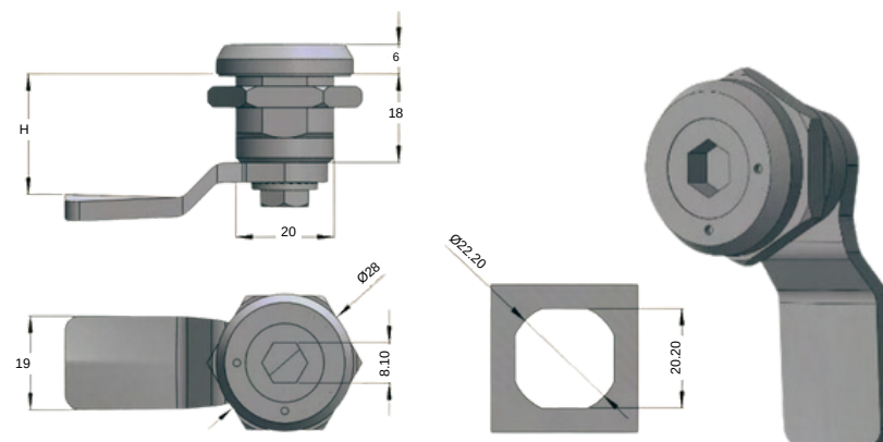
STAINLESS STEEL QUARTER TURN 2514-HT-6.1
