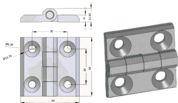
STAINLESS STEEL HINGE 2715-HT-5.1
