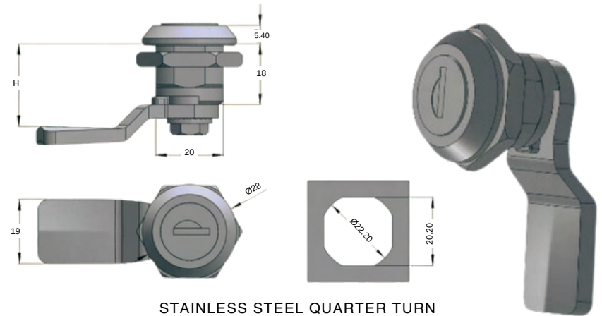
STAINLESS STEEL QUARTER TURN 2513-HT-1.2
