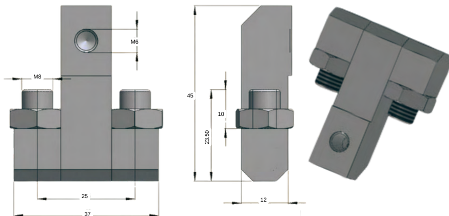
STAINLESS STEEL HINGE 3140-HT-1.8
