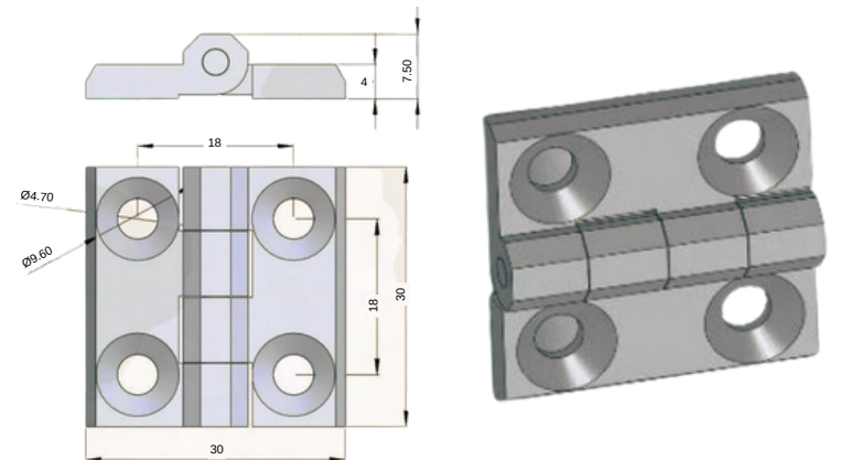
STAINLESS STEEL HINGE 2715-HT-3.1
