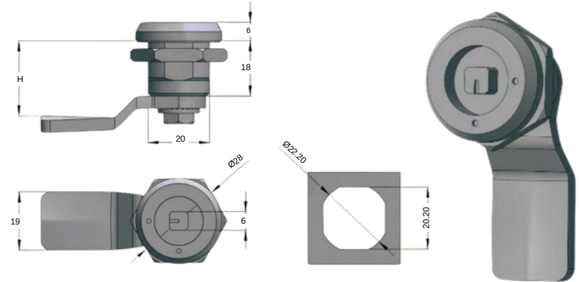
STAINLESS STEEL QUARTER TURN 2514-HT-4.1
