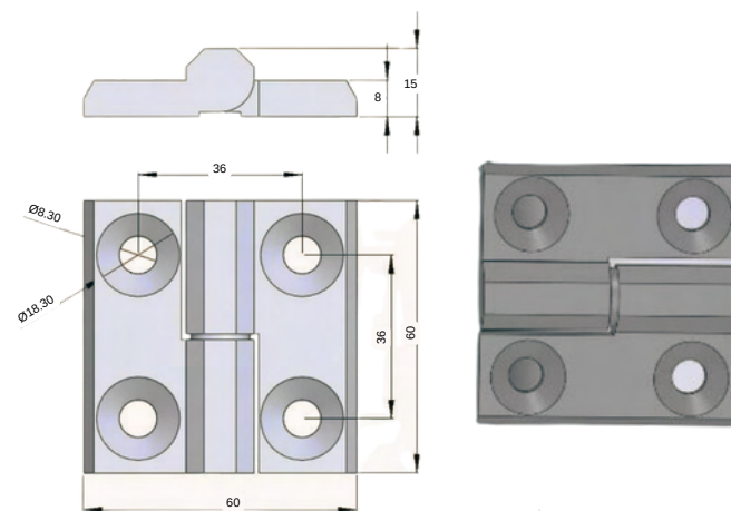
STAINLESS STEEL HINGE 2715-HT-6.4
