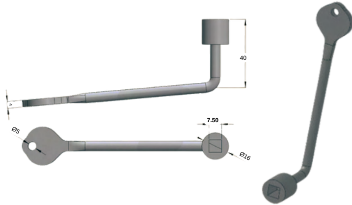
STAINLESS STEEL KEY
