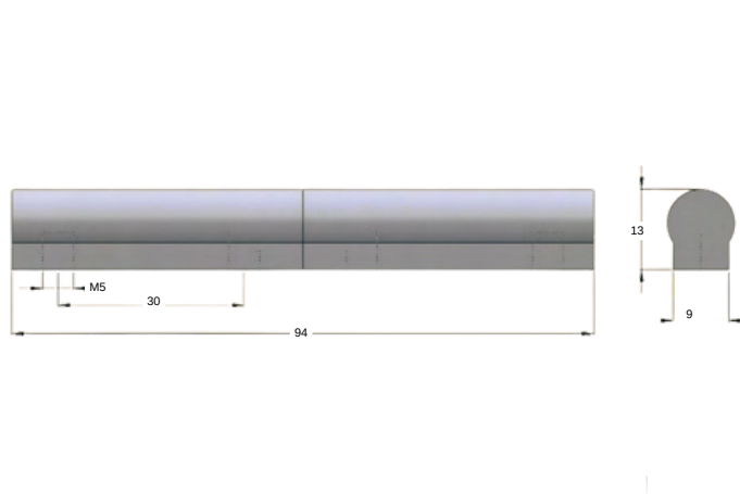
STAINLESS STEEL HINGE 3140-HT-1.4
