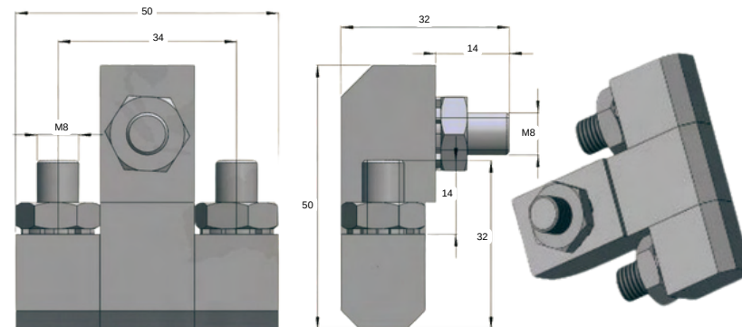
STAINLESS STEEL HINGE 3140-HT-1.9
