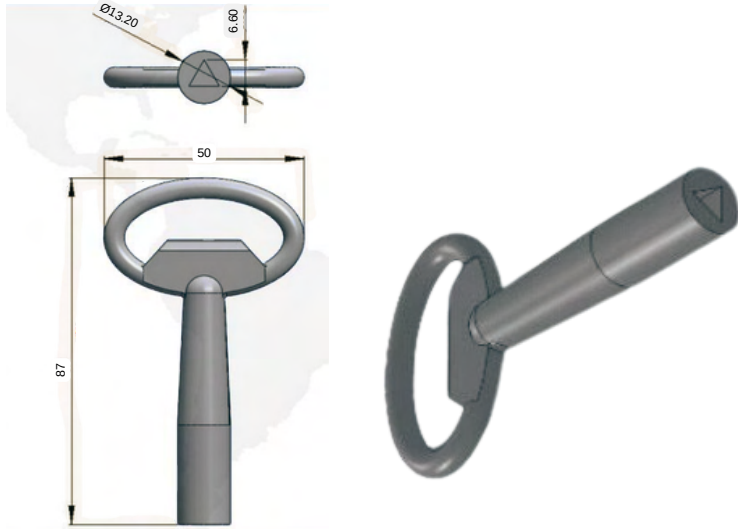
STAINLESS STEEL KEY
