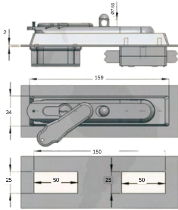
ZINC DIE-CAST CYLINDER 1810-HT-2.1
