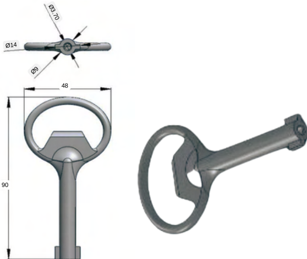
STAINLESS STEEL KEY
