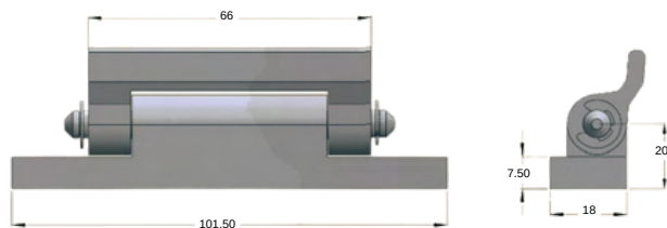
STAINLESS STEEL HINGE 3140-HT-1.26
