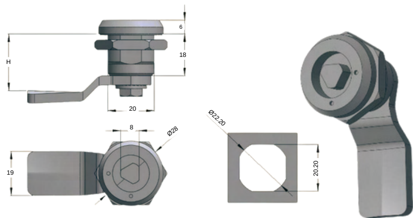
STAINLESS STEEL QUARTER TURN 2514-HT-3.2
