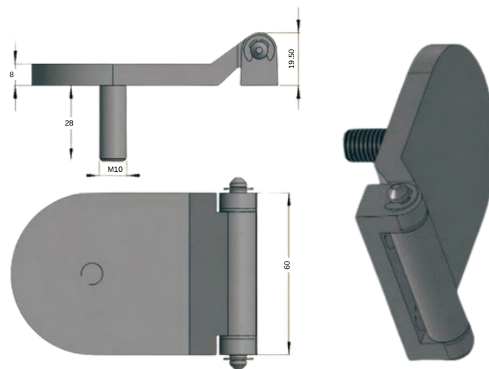
STAINLESS STEEL HINGE 3140-HT-1.25
