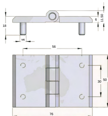
STAINLESS STEEL HINGE 2715-HT-5.7
